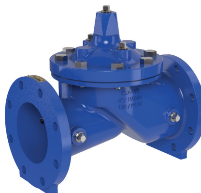
Model 100-20 Reduced Port Hytrol Main Valve
