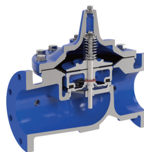
Model 100-01 Full Port Hytrol Main Valve
